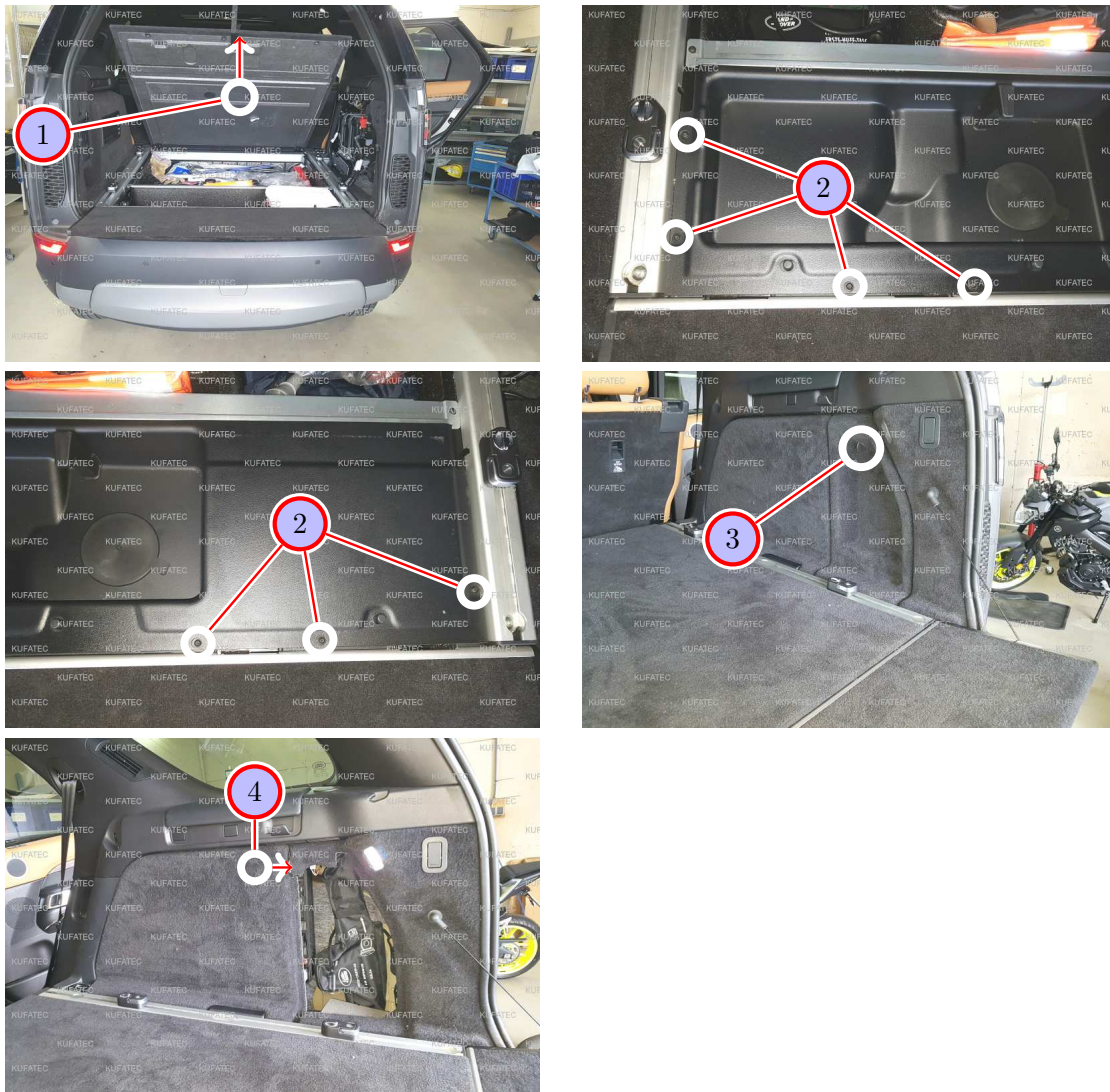
Figure 6: Removing trunk trim panels
